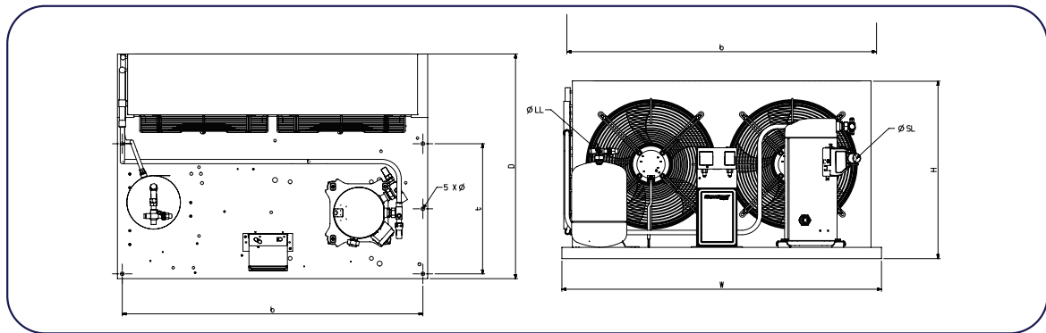
Medium temperature double fan model
