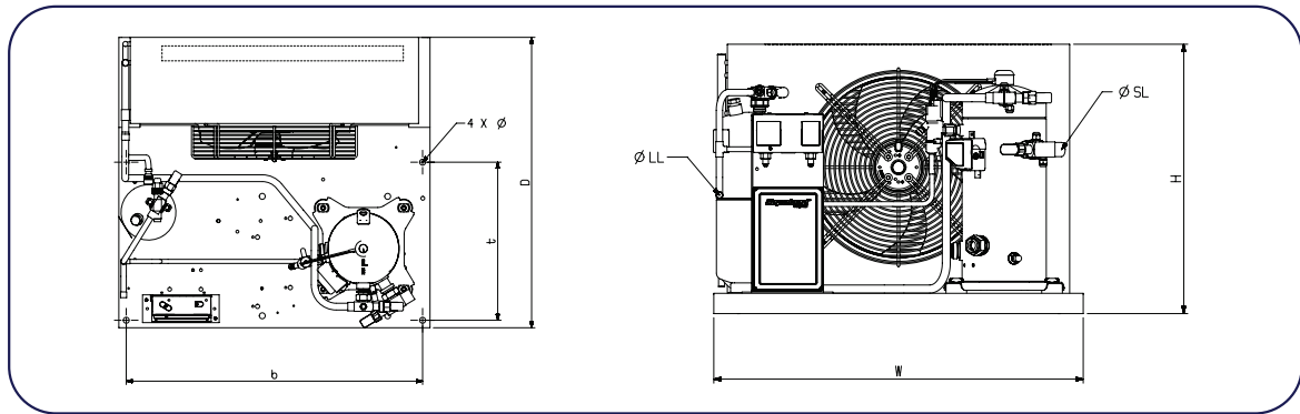
Low temperature single fan model
